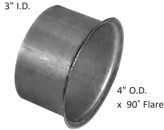
9479 Replaces GMC Part No.2046594 Extension Requires 9611 V-Clamp
