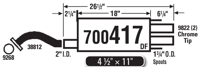
4/99-03 Maxima (exc. CA)
