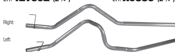
02-05 DODGE Ram 1500/2500 (Under 8800 lbs. GVW); 6 & 8 Cyl; 3.7L, 4.7L; 120" WB; Dual Conversion
