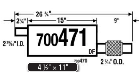
04-06 Chrysler, Pacifica, V6-3.5L, Front Muffler
