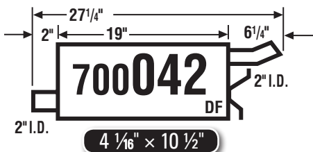
92-94 Crown Victoria, Grand Marquis Sedan, Sgl. Exh., Dual Exh. (Right) 90-94 Town Car, Sgl. Exh., Dual Exh. (Right)
