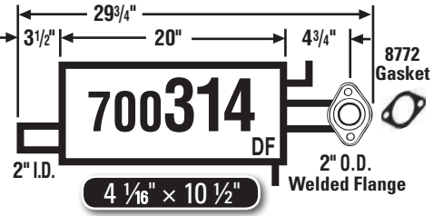
98-02 Full Size Models, Sgl. Exh, Dual Exh. (Right)
