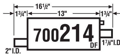
93-94 Chev. Lumina, Dual Exh. (Left) 93-96 Grand Prix, Dual Exh. (Left)
