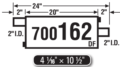
92-94 Skylark, Achieva, Grand AM 93-94 Beretta, Corsica, exc. Beretta GT/GTZ, Z26
