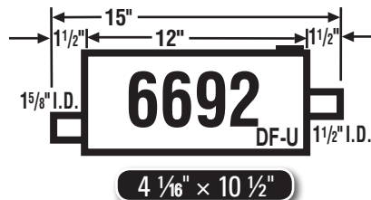
87-93 Sentra; Sedan, 2 W.D. Wagon
