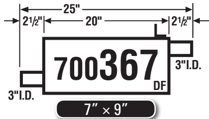
99-04 F250, F350, Super Duty
