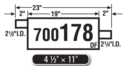
92-94 Bravada 4 WD 92-94 Blazer/Jimmy 2 WD (S10/S15), 4 WD (T10/T15)
