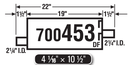
00-01 Explorer, 4.0L., 4-Dr. (From 12/99) 00-03 Explorer Sport, 4.0L., 2-Dr. (From 12/99)
