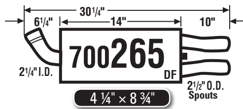
85-90 Corvette, exc. ZR1, Dual Exh. (Left)
