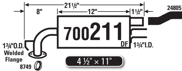
93-97 Geo Prizm, Prizm LSI (Welded Assembly Available)
