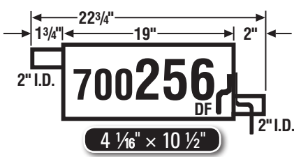
96-99 Taurus, Sable, Sgl. Exh., Dual Exh. (Left)
