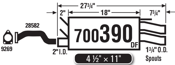
95-00 Avenger, Sebring LX, LXI Coupe
