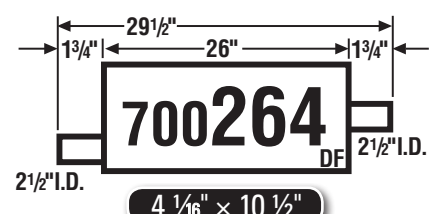
76-78 B100, BF100, B200, BF200, B300, BF300, CB300, MB300, MB400, PB100, PB200, PB300
