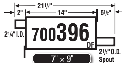
01-10 PT Cruiser (exc. Turbo)
