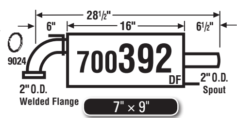
98-02 Accord, DX, LX, EX, SE
