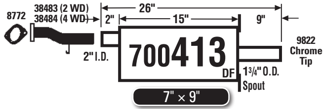
96-99 Legacy Outback 94-99 Legacy Sta. Wagon, 2.2L
