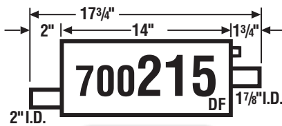
1993 Cutlass Supreme, Dual Exh. (Right) 93-96 Grand Prix, Dual Exh. (Right)
