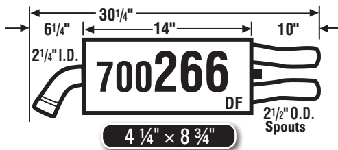
85-90 Corvette, exc. ZR1, Dual Exh. (Right)
