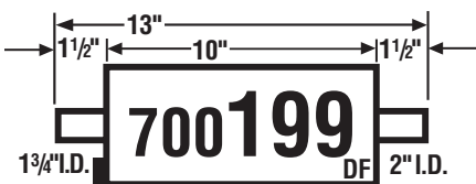
92-94 Achieva, Grand AM (Right)
