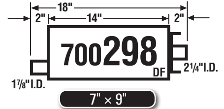
00-05 Monte Carlo, Dual Exh. (Right) 97-08 Grand Prix, Dual Exh. (Right) 05-08 Lacrosse, Dual Exh. (Right) 05-07 Allure, Dual Exh. (Right)
