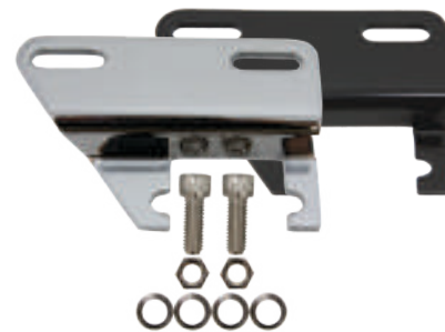
CHEVY SMALL BLOCK - SWP ALTERNATOR BRACKET F STYLE 1955-68 289-302 HZ-9323-C Chrome HZ-9323-PBK Black Slide Driver Side Only
