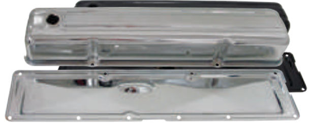
CHEVY STRAIGHT 6 - SMOOTH 1952-62, 236-L6 UNBAFFLED
