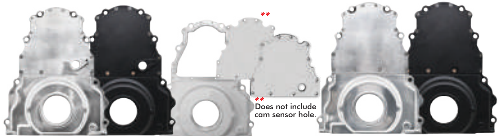
LS Timing Cover Two Piece without Cam Sensor Hole
