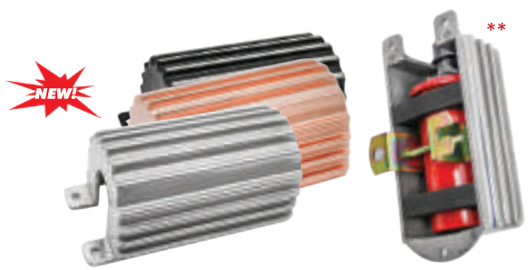
ALUMINUM FINNED CANNISTER ROUND IGNITION COIL COVER HZ-2045-POL Polished HZ-2045-POL-KIT Polished** HZ-2045-PBK Black HZ-2045-PBK-KIT Black** HZ-2045-COP Copper HZ-2045-COP-KIT Copper**
