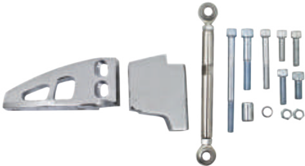
CHEVY SMALL BLOCK - SWP AIR CONDITIONING BRACKET - ALUMINUM 262-267-283-305-327-350-400
