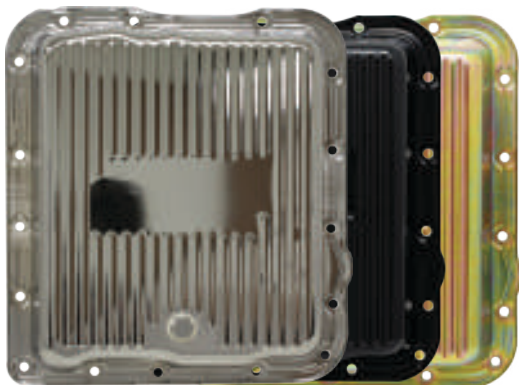
CHEVY/GM 700R4-4L60E-4L65E HZ-7599-C Chrome HZ-9712-C Chrome HZ-7599-PBK Black HZ-9712-PBK Black HZ-7599-Z Zinc HZ-9712-Z Zinc DEPTH: 2-5/8" DEPTH: 3-5/8"
