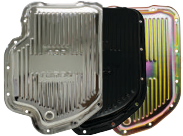
CHEVY/GM TH-400 HZ-9121-C Chrome HZ-9197-C Chrome HZ-9121-PBK Black HZ-9197-PBK Black HZ-9121-Z Zinc HZ-9197-Z Zinc DEPTH: 2" DEPTH: 3"
