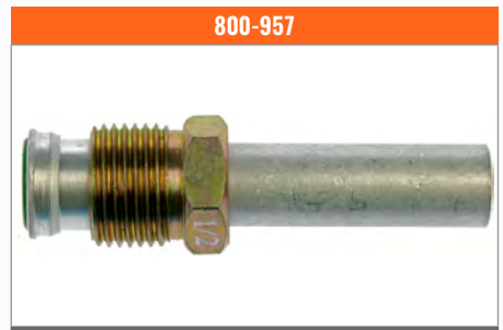
800-957 Tube End 1/2 In. Female Tube End 3/4 In. - 16 External Thread Nut
